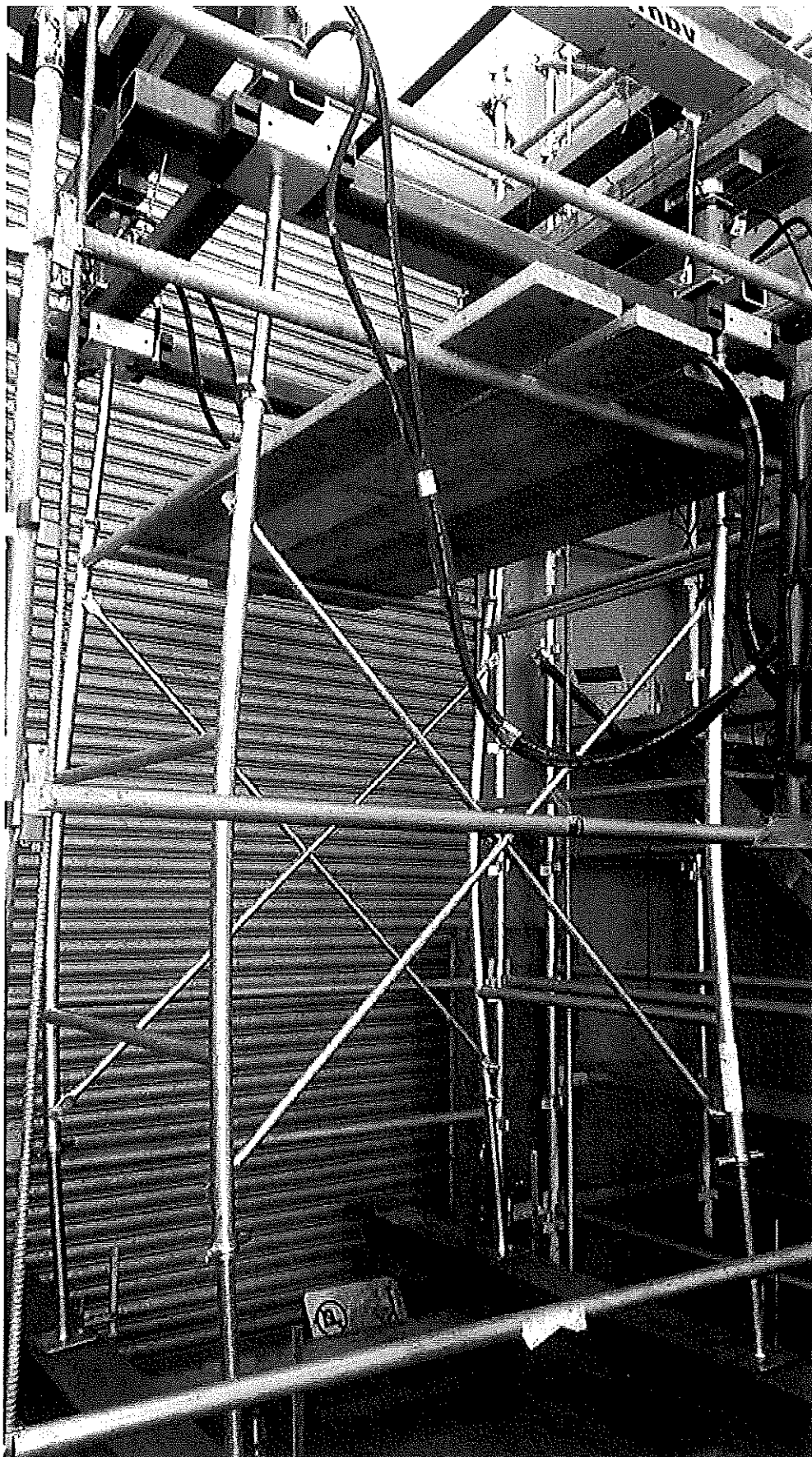
Photo C: The assembly under load with eccentric arrangement
